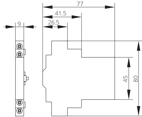
Auxiliary switch PS
