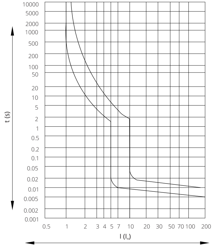
I_n < 10 \text{ A} Characteristics C acc. to EN 60 898
