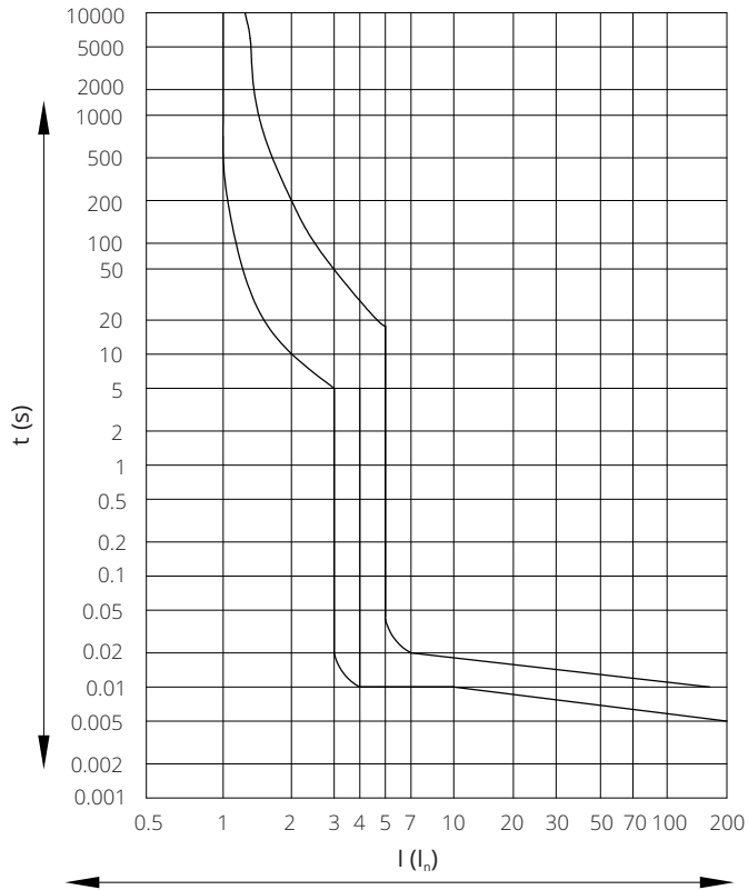
I_n \geq 10 \text{ A} Characteristics B acc. to EN 60 898
